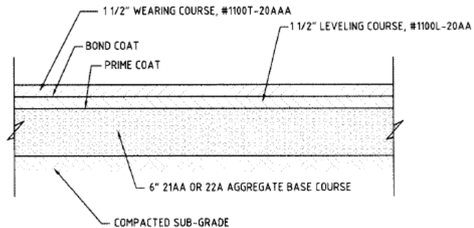
BITUMINOUS PAVEMENT DETAIL SCALE: NONE
