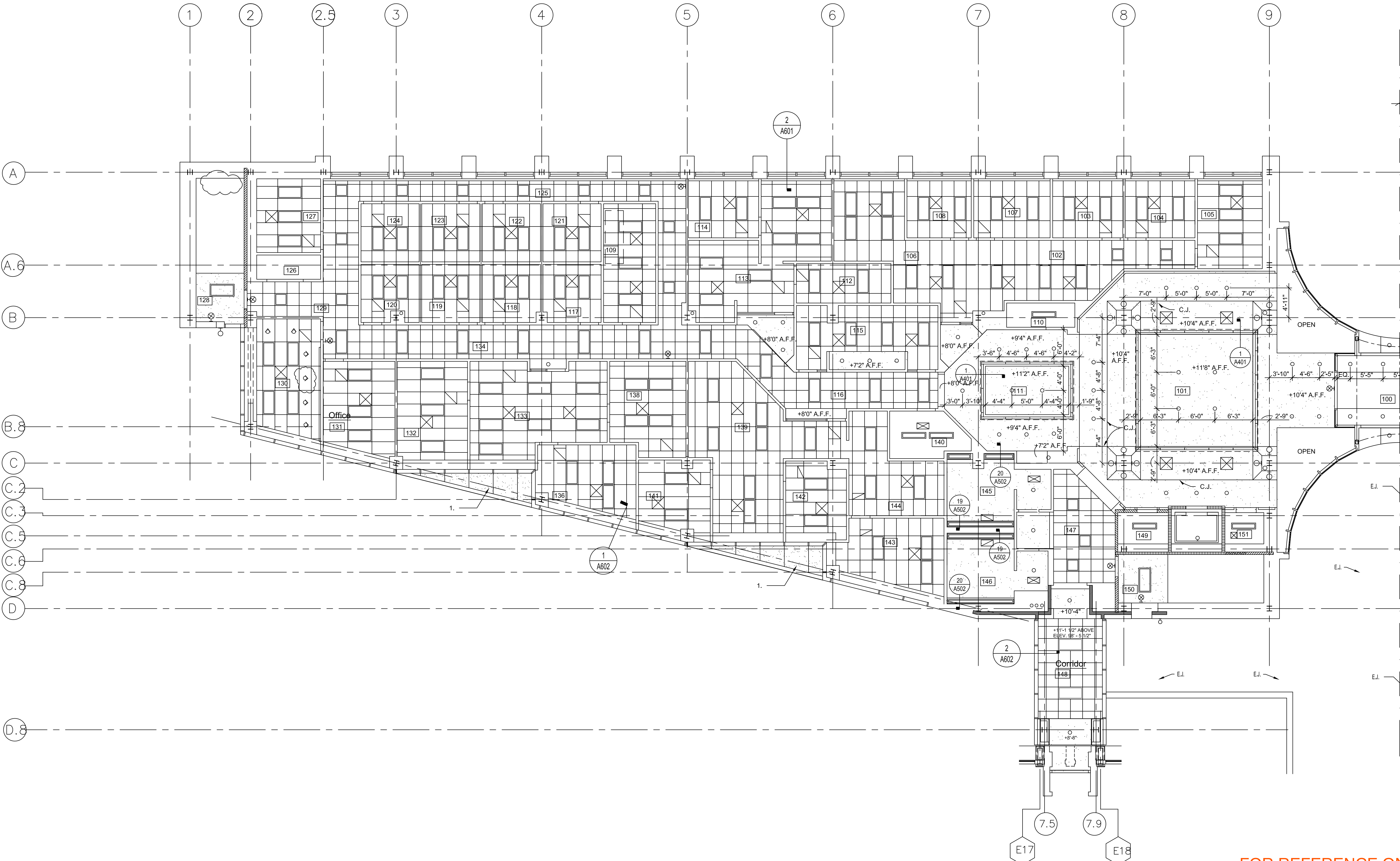
Reflected Ceiling Plan Level One Addition West 1/8"=1'-0"
