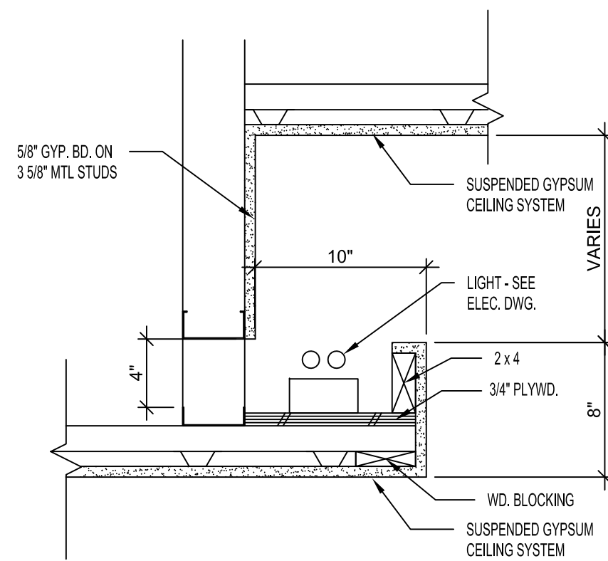
Light Shelf Detail
