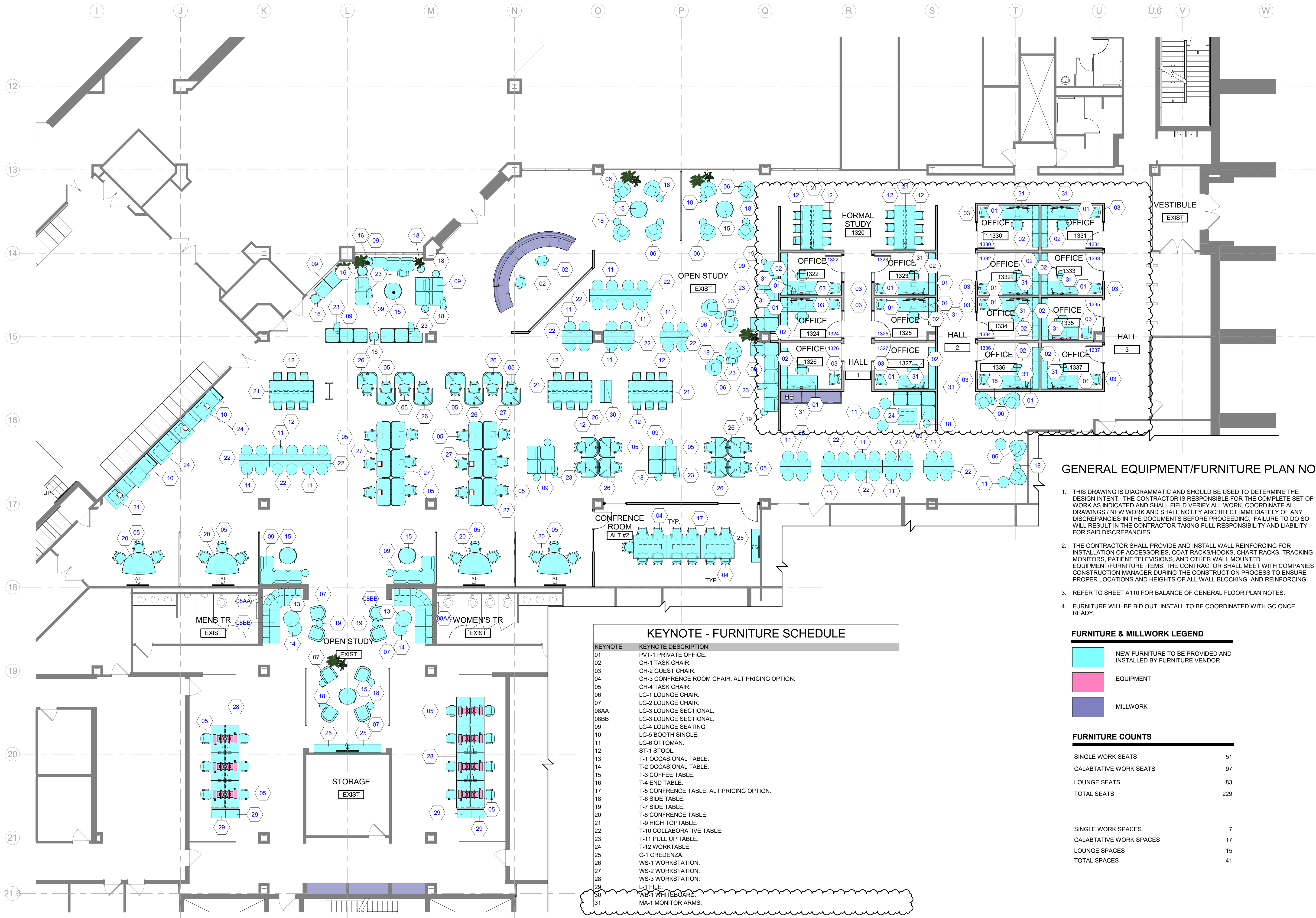
1 FURNIUTRE FLOOR PLAN 1/8" = 1'-0"
